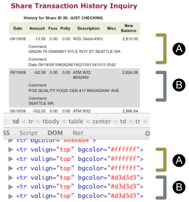
Figure 8: The bank account internals as displayed in Firebug. Notice that each tuple spans multiple <tr> nodes of varying background color, without a single enclosing parent. XPath expressions segment each element of a list along an enclosing parent, which fails when a tuple is composed of multiple children. They also have trouble when there are extraneous children or when tuples are at different depths in the tree.
